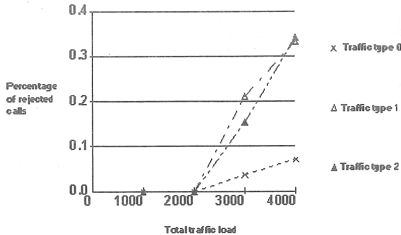
Fig. 3: Percentage of rejected calls versus total traffic load for the complete sharing and priority strategies.
