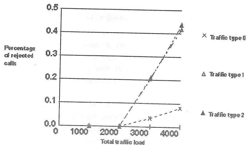
Fig. 2: Percentage of rejected calls versus total traffic load for the complete sharing and cyclic strategies.
