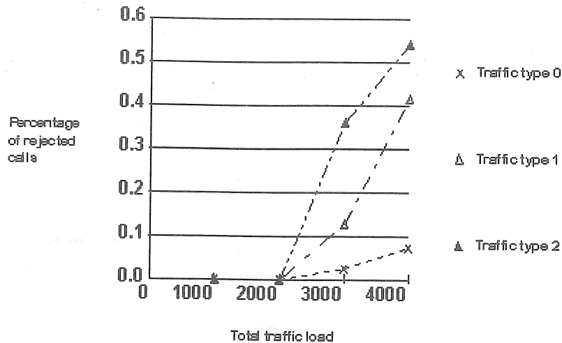
Fig. 5: Percentage of rejected calls versus total traffic load for the movable boundary and cyclic strategies.
