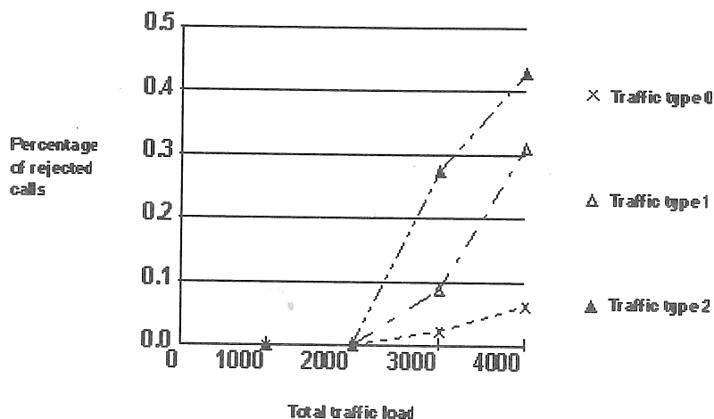
Fig. 6: Percentage of rejected calls versus total traffic load for the movable boundary and priority strategies.
