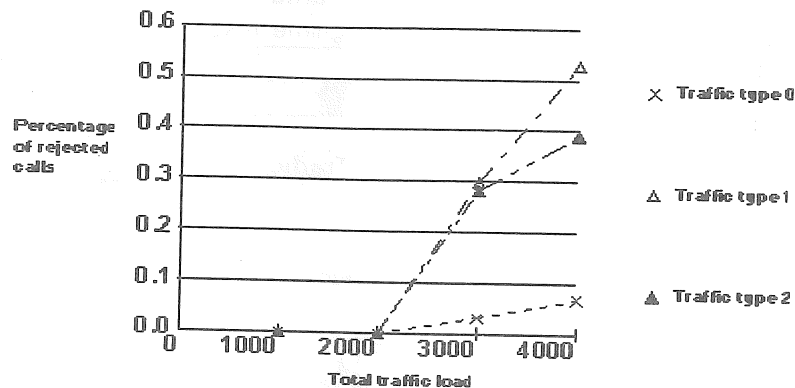
Fig. 1: Percentage of rejected calls versus total traffic load for the complete sharing and FIFO strategies.
