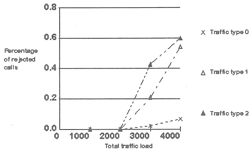
Fig. 4: Percentage of rejected calls versus total traffic load for the movable boundary and FIFO strategies.
